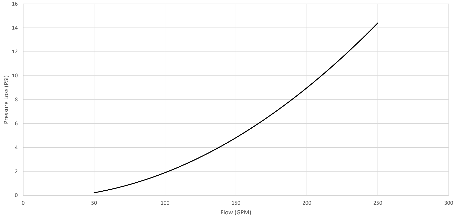
555A Pressure Loss
